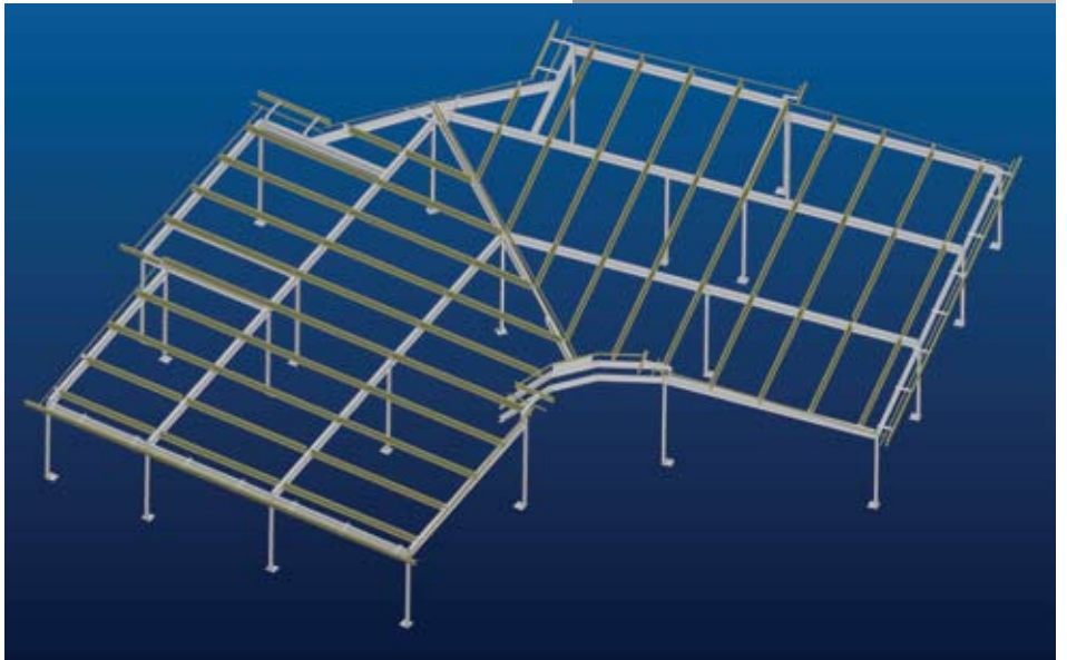
Structural roof.
