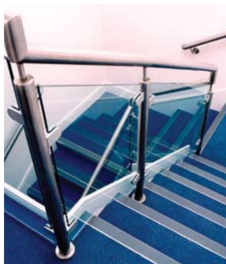
All stainless steel with rose cover floor plates and preparatory glazing brackets
